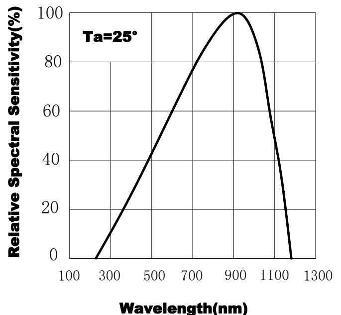
Fig.2 Spectral Sensitivity
