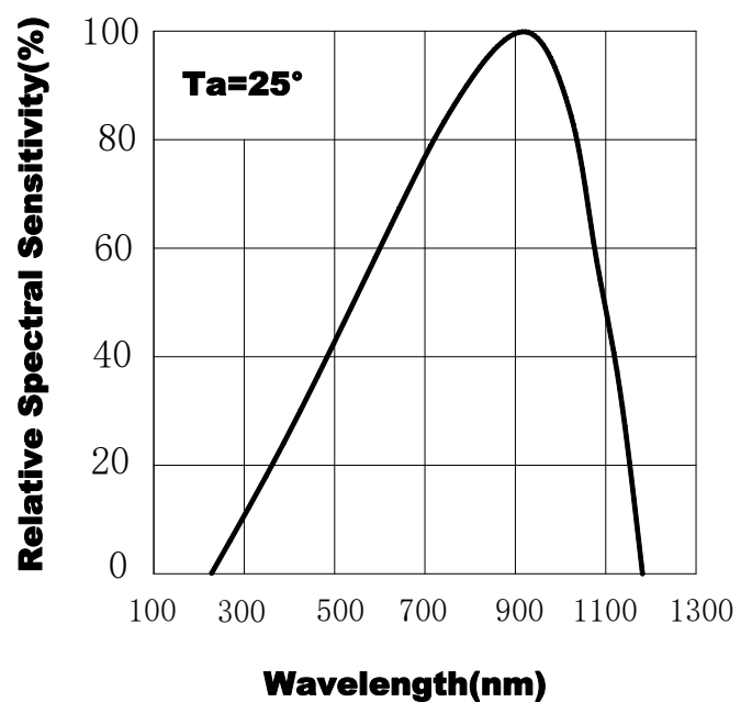
Fig.2 Spectral Sensitivity
