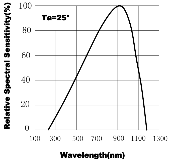
Fig.2 Spectral Sensitivity
