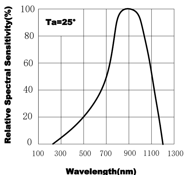
Fig.2 Spectral Sensitivity
