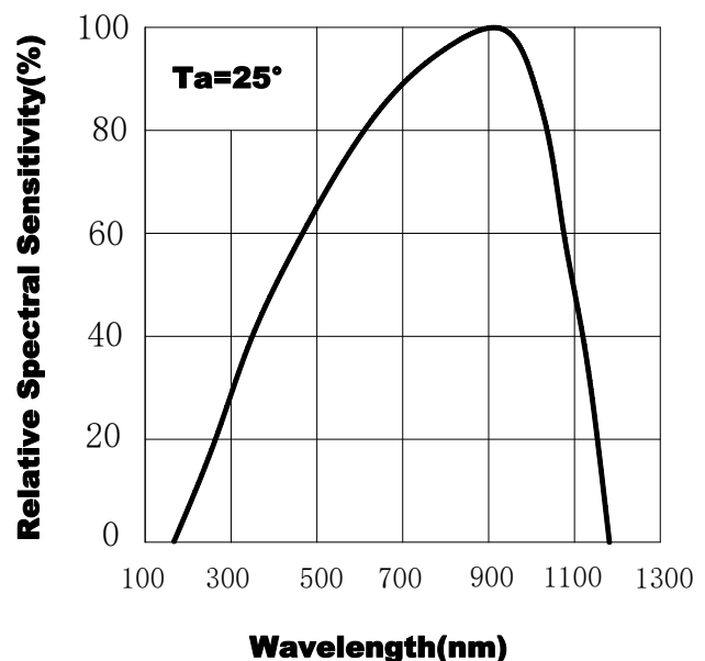
Fig.2 Spectral Sensitivity
