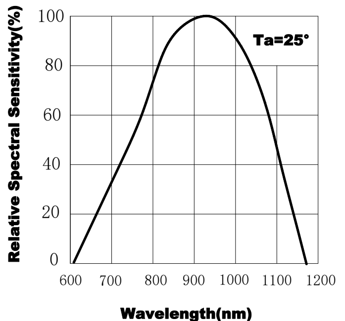
Fig.2 Spectral Sensitivity
