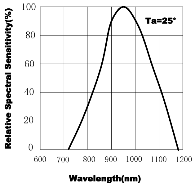
Fig.2 Spectral Sensitivity
