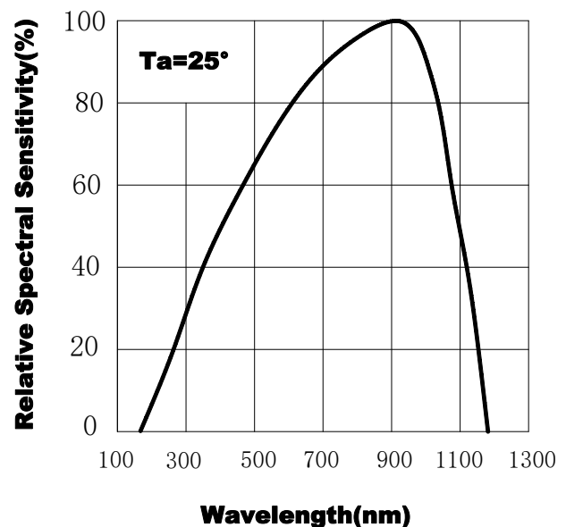
Fig.2 Spectral Sensitivity
