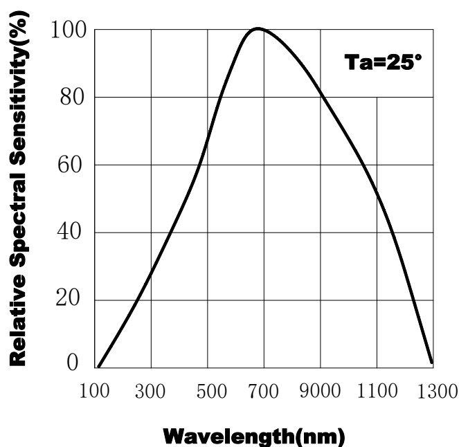
Fig.2 Spectral Sensitivity
