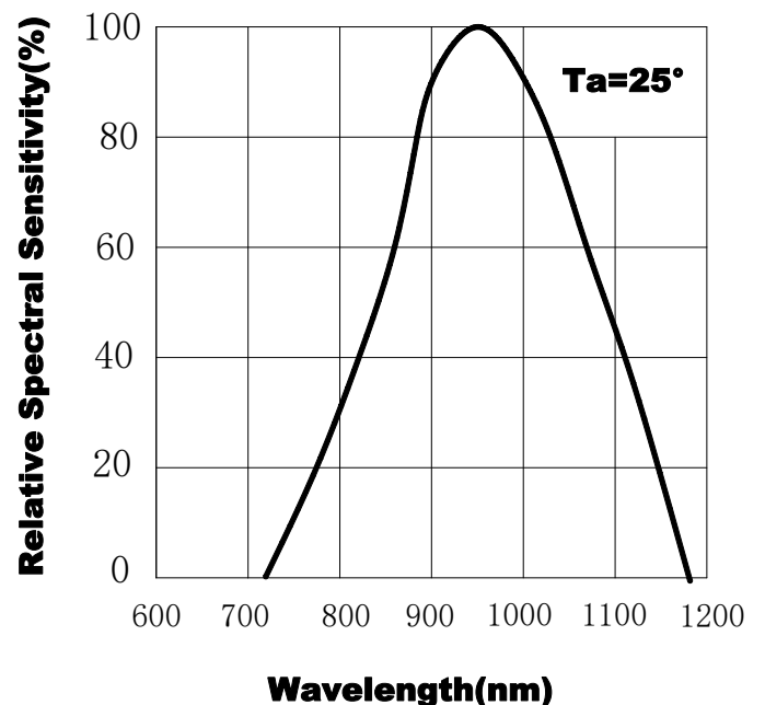
Fig.2 Spectral Sensitivity
