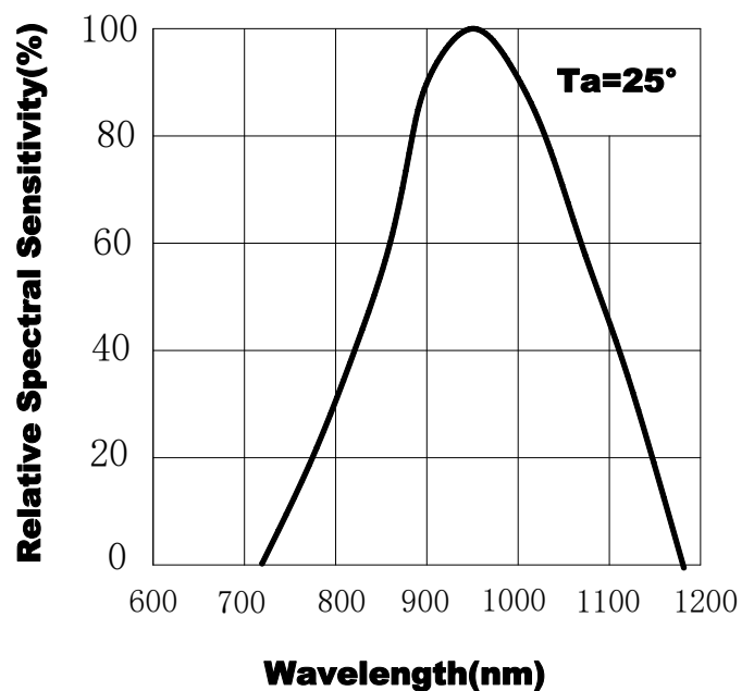
Fig.2 Spectral Sensitivity
