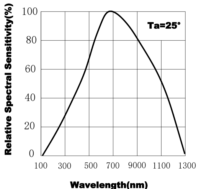
Fig.2 Spectral Sensitivity
