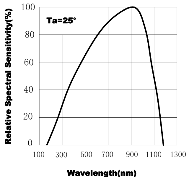
Fig.2 Spectral Sensitivity
