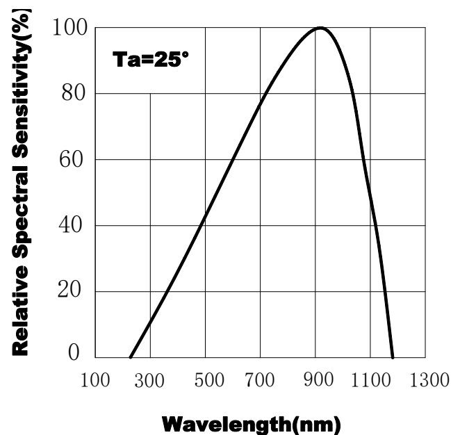
Fig.2 Spectral Sensitivity
