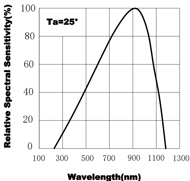
Fig.2 Spectral Sensitivity
