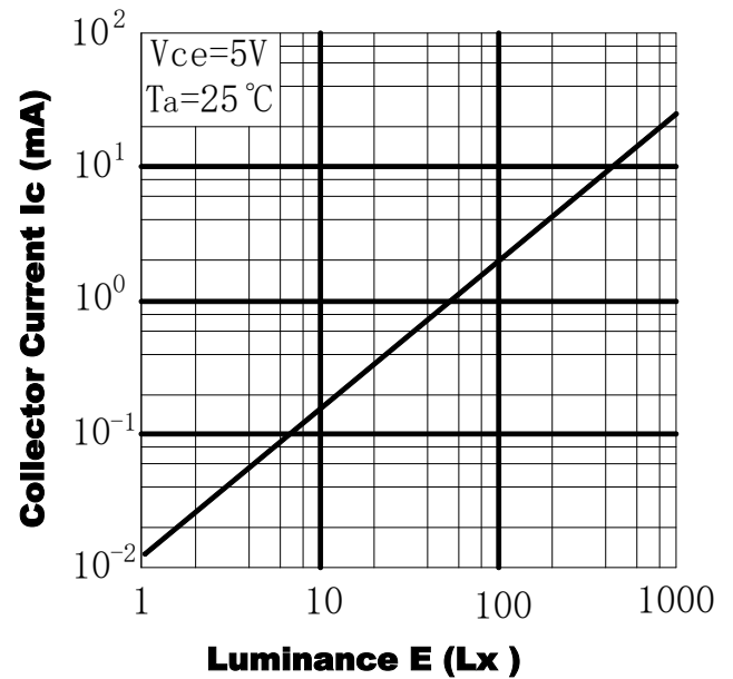
Fig.4 Collector Current vs. Luminance
