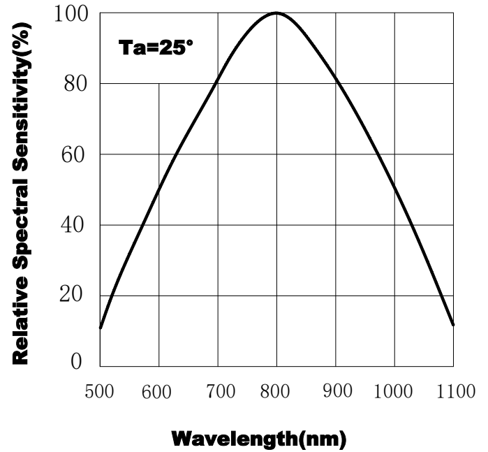
Fig.2 Spectral Sensitivity
