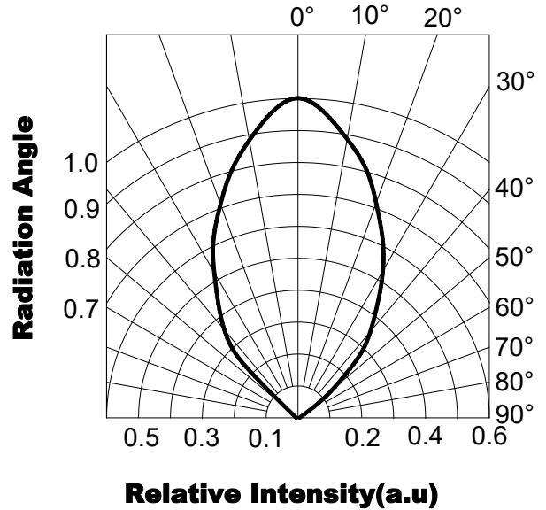
Directivity (Ta=25°C)
