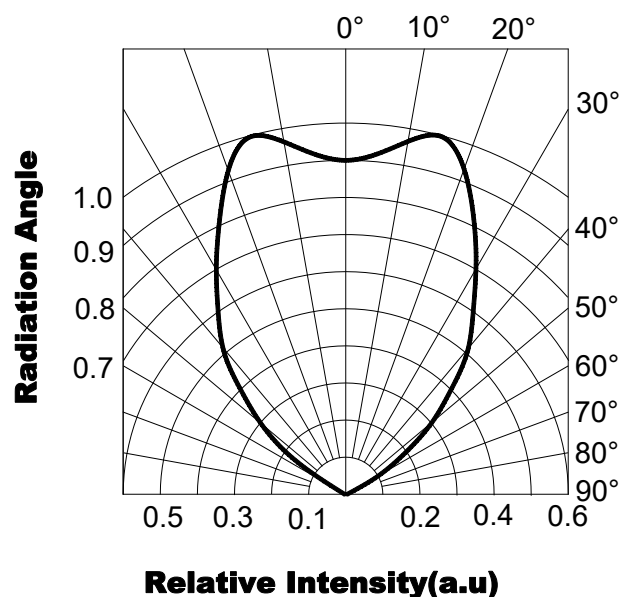
Directivity (Ta=25°C)
