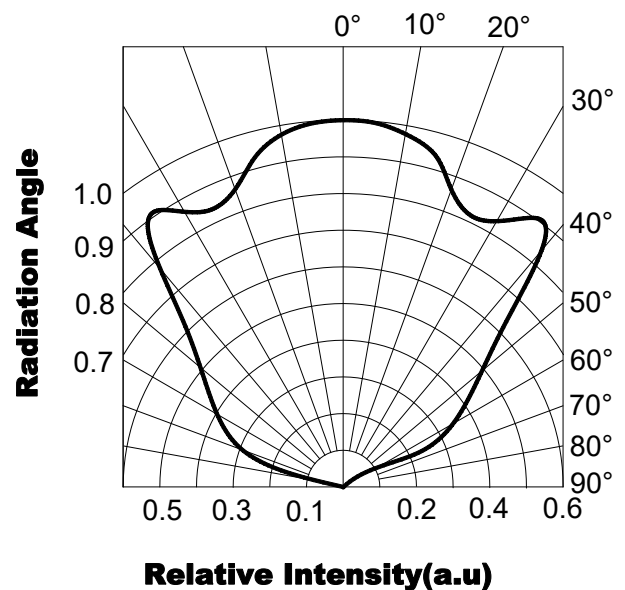
Directivity (Ta=25°C)
