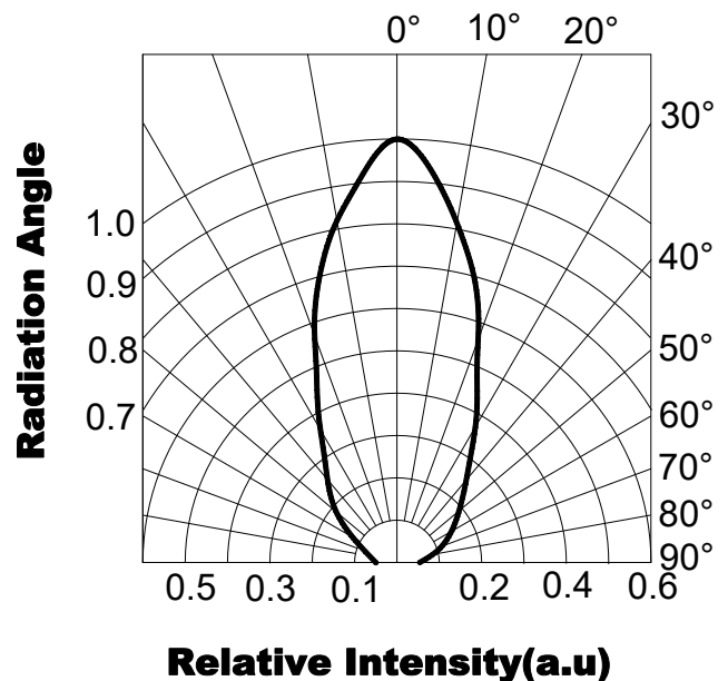
Directivity (Ta=25°C)
