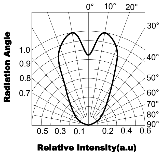
Directivity (Ta=25°C)
