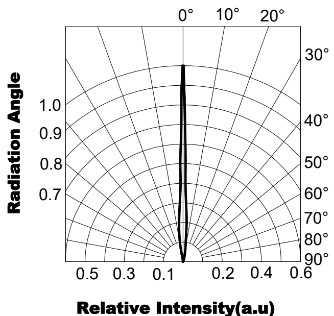
Directivity (Ta=25°C)
