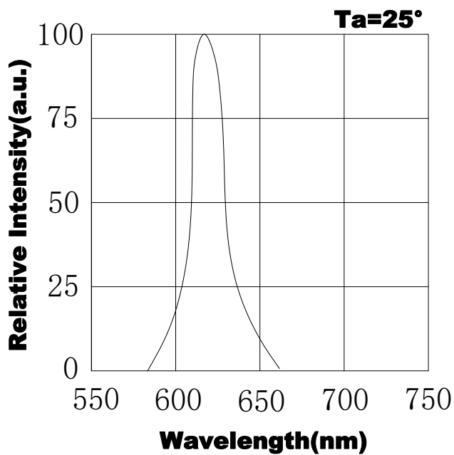
Relative Intensity vs. Wavelength (Ta=25°C)
