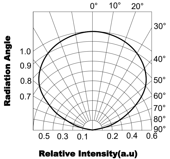
Directivity (Ta=25°C)
